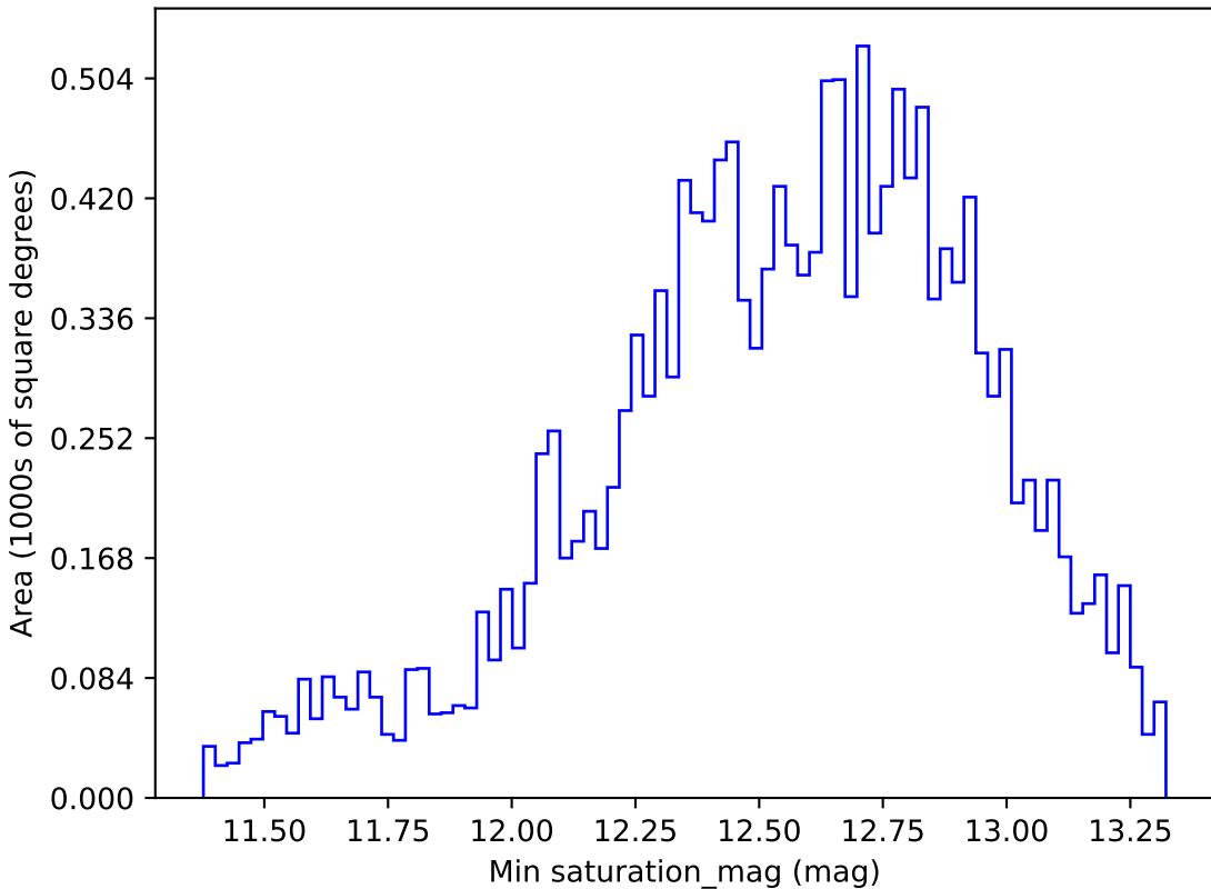
ddf_half_v3.4_10yrs WFD r band: Min saturation_mag
