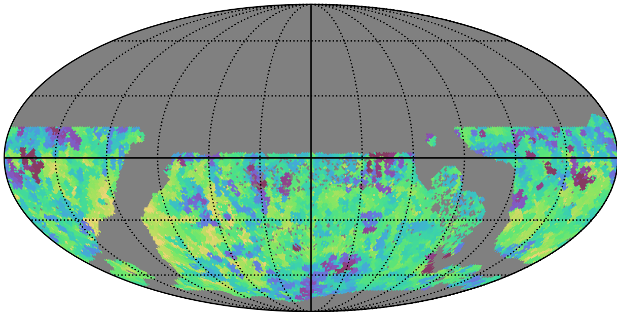
ddf_half_v3.4_10yrs WFD i band: Min saturation_mag
