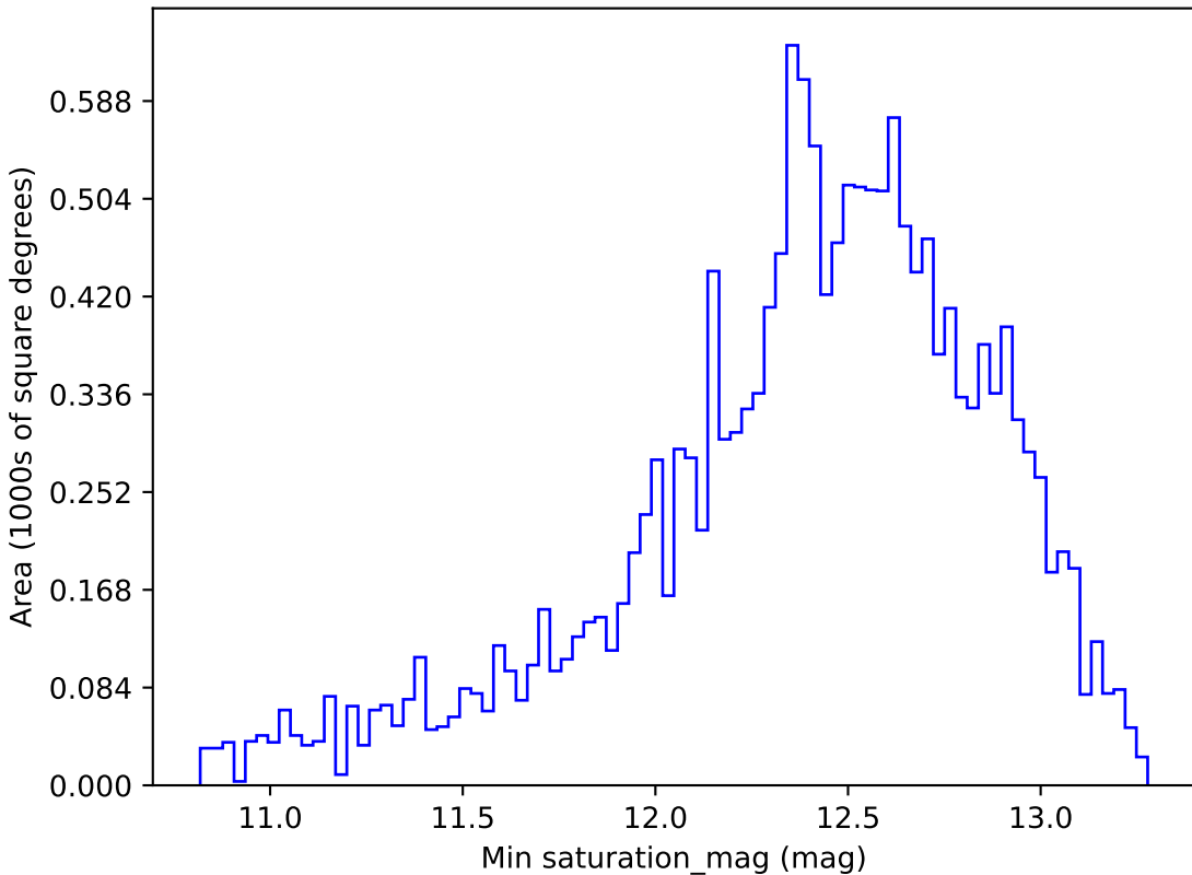
ddf_half_v3.4_10yrs WFD i band: Min saturation_mag
