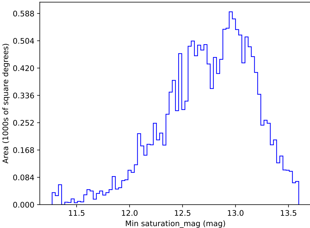
ddf_half_v3.4_10yrs WFD g band: Min saturation_mag
