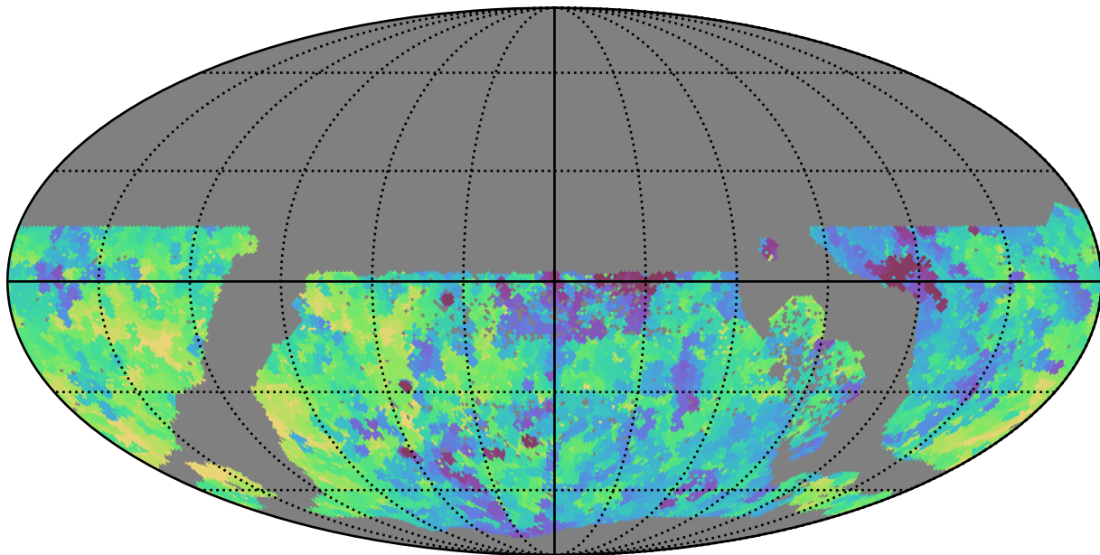
ddf_half_v3.4_10yrs WFD all bands: Min saturation_mag
