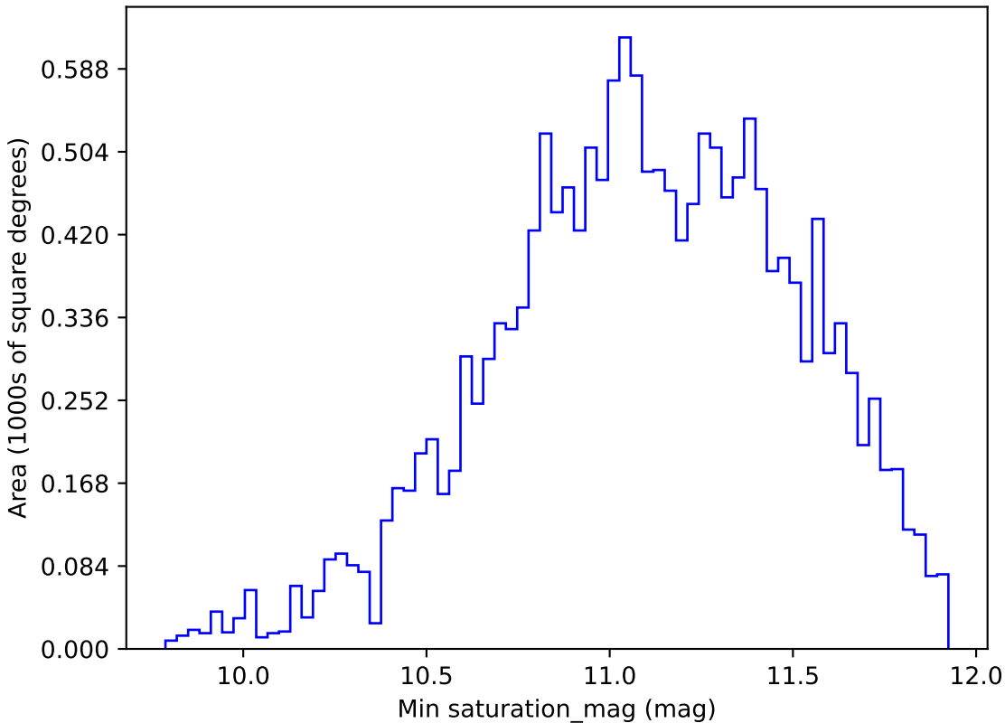
ddf_half_v3.4_10yrs WFD all bands: Min saturation_mag
