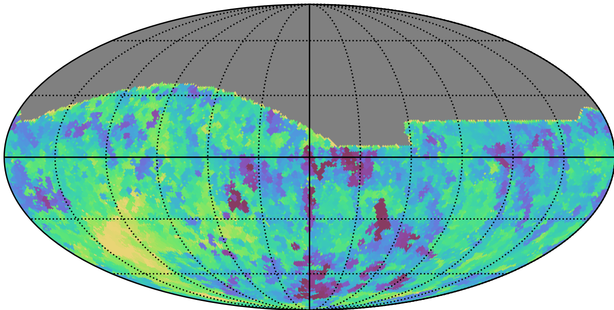
ddf_half_v3.4_10yrs All sky z band: Min saturation_mag
