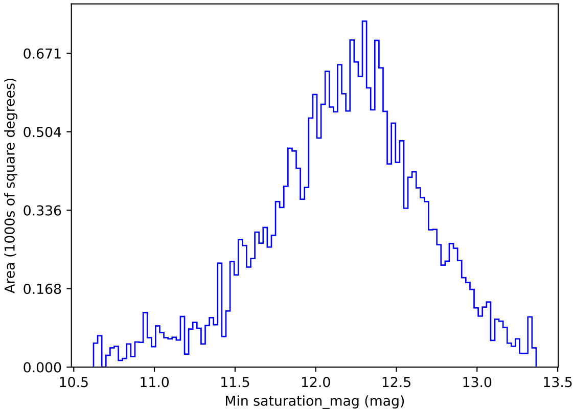
ddf_half_v3.4_10yrs All sky z band: Min saturation_mag
