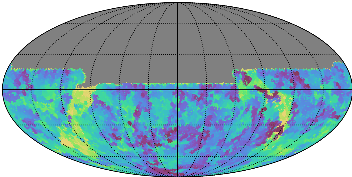
ddf_half_v3.4_10yrs All sky u band: Min saturation_mag
