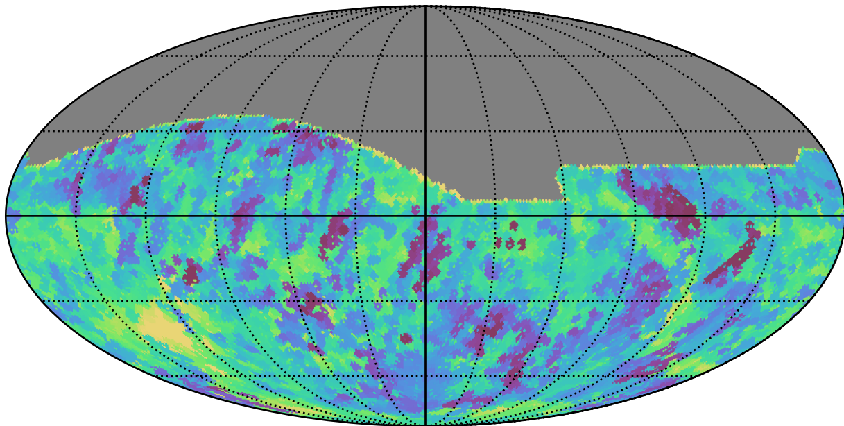
ddf_half_v3.4_10yrs All sky r band: Min saturation_mag
