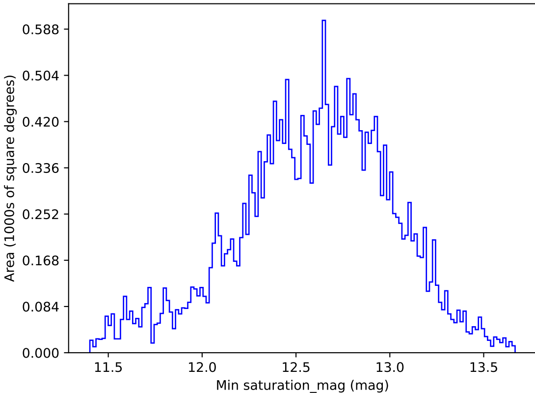
ddf_half_v3.4_10yrs All sky r band: Min saturation_mag
