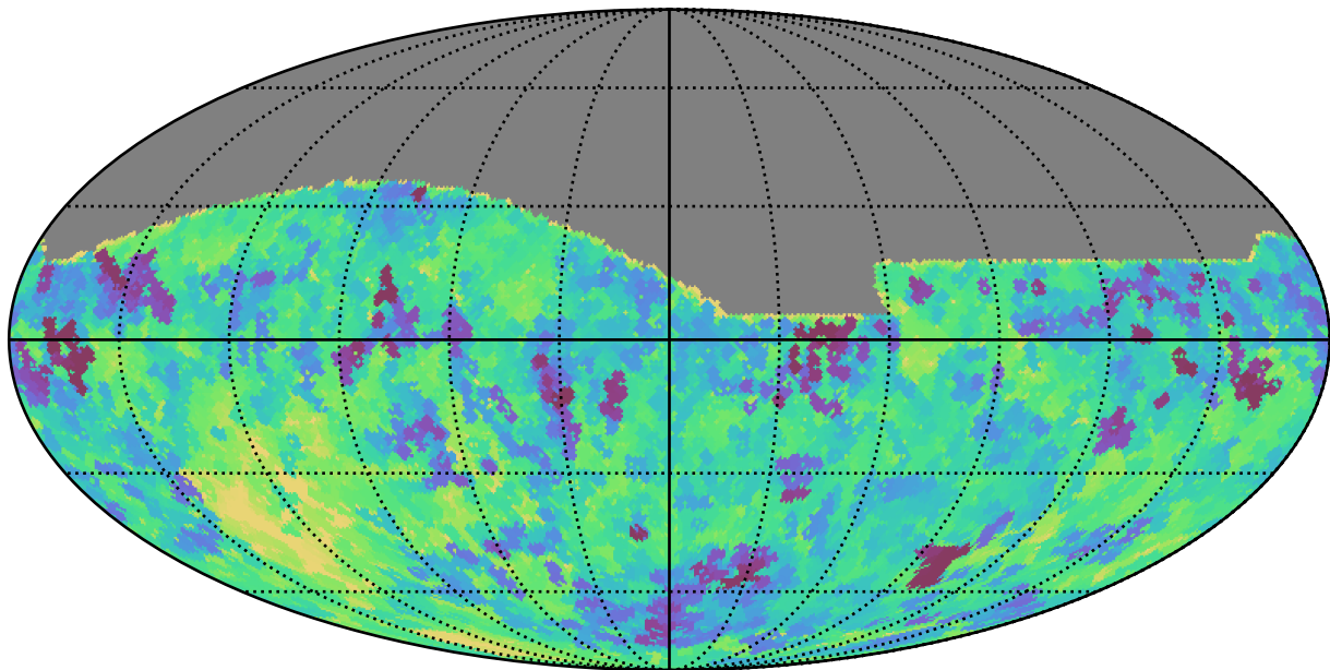
ddf_half_v3.4_10yrs All sky i band: Min saturation_mag
