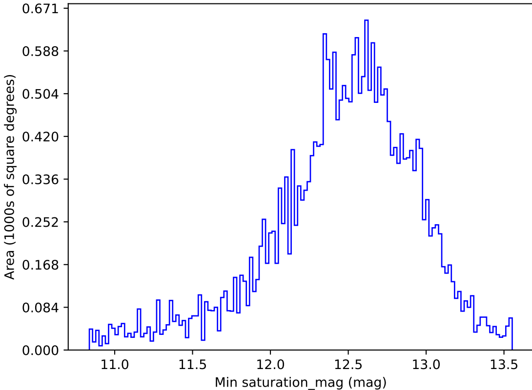
ddf_half_v3.4_10yrs All sky i band: Min saturation_mag
