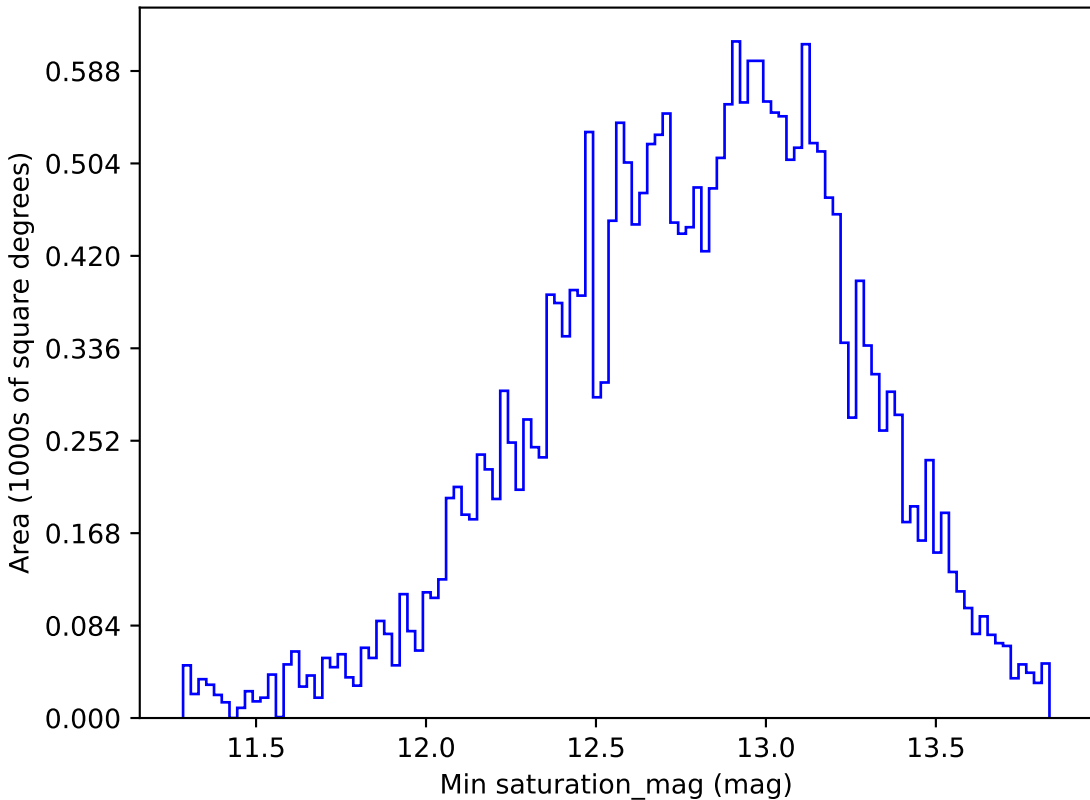
ddf_half_v3.4_10yrs All sky g band: Min saturation_mag
