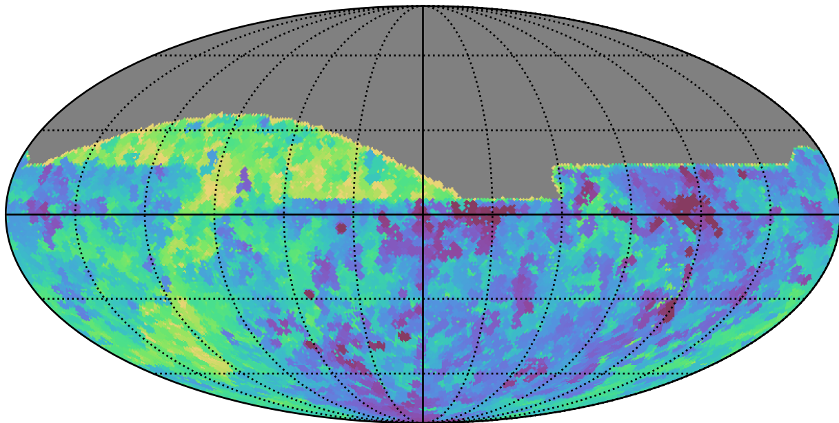
ddf_half_v3.4_10yrs All sky all bands: Min saturation_mag
