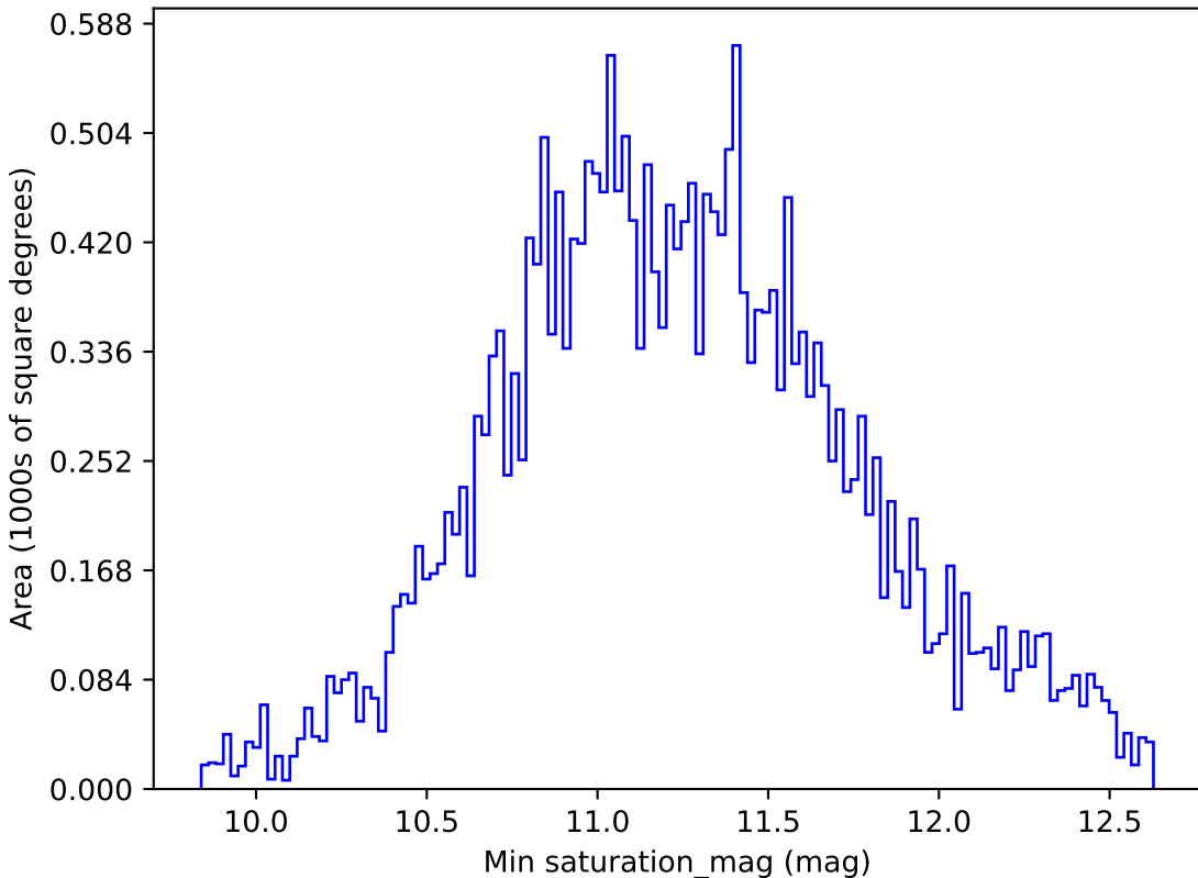
ddf_half_v3.4_10yrs All sky all bands: Min saturation_mag
