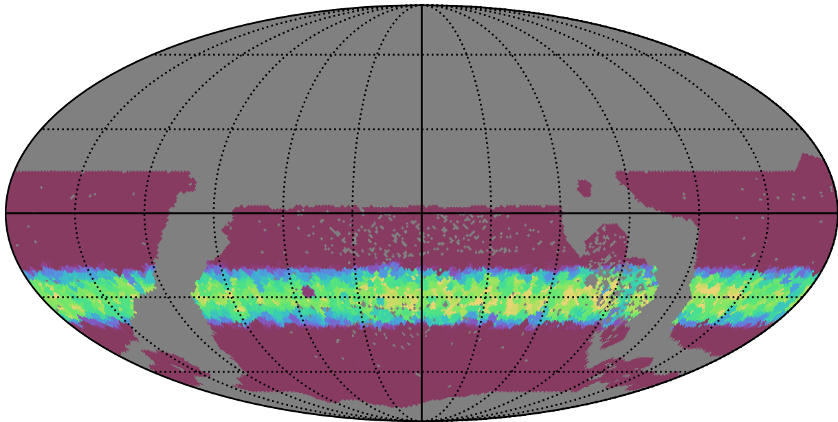
ddf_half_v3.4_10yrs WFD z band: Min normairmass
