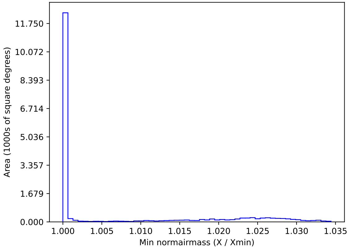
ddf_half_v3.4_10yrs WFD z band: Min normairmass
