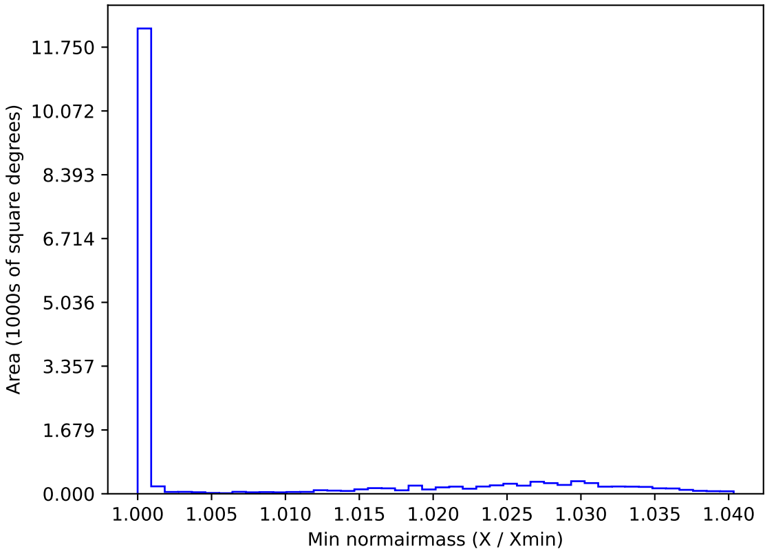
ddf_half_v3.4_10yrs WFD y band: Min normairmass
