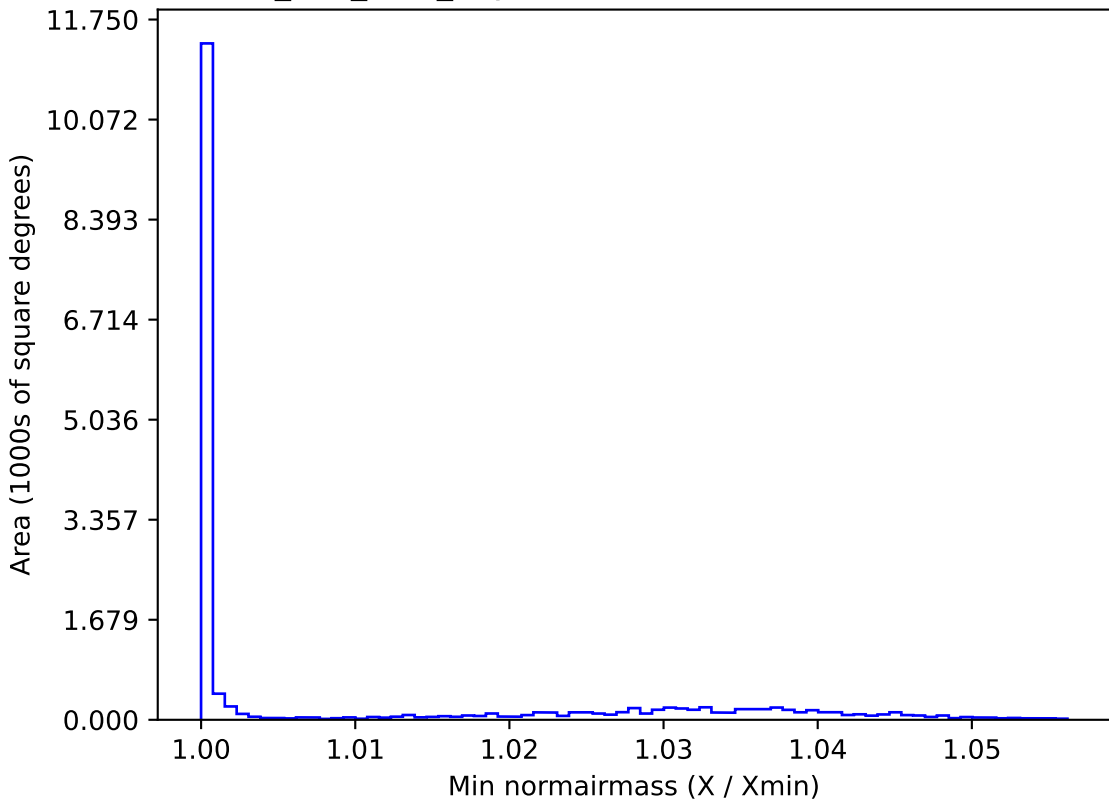
ddf_half_v3.4_10yrs WFD u band: Min normairmass
