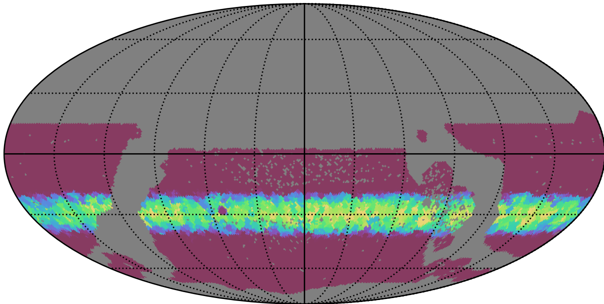
ddf_half_v3.4_10yrs WFD r band: Min normairmass
