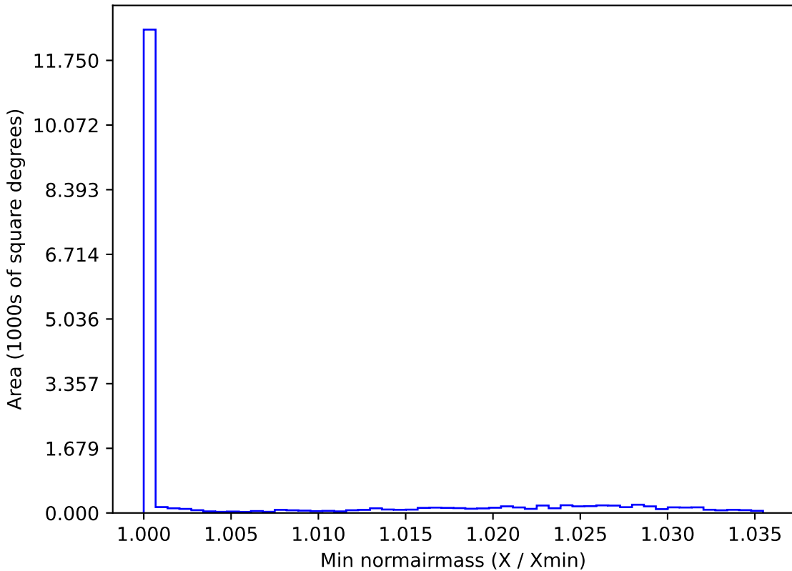
ddf_half_v3.4_10yrs WFD r band: Min normairmass
