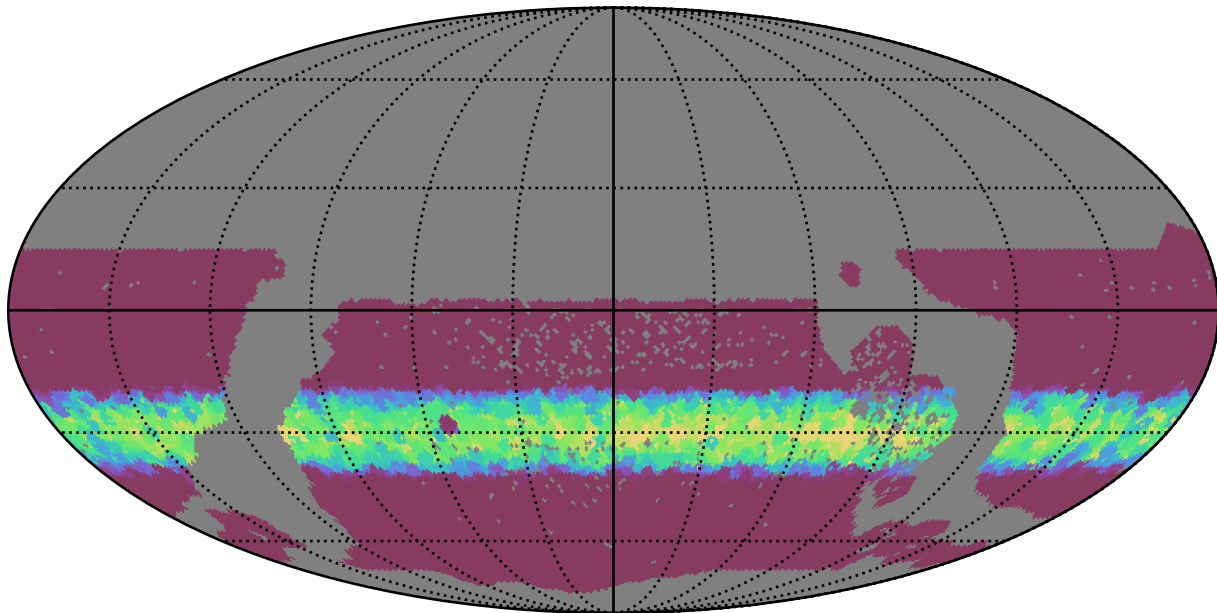
ddf_half_v3.4_10yrs WFD i band: Min normairmass
