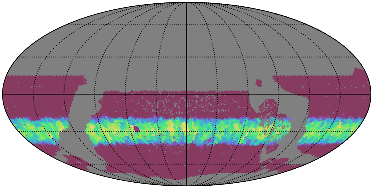
ddf_half_v3.4_10yrs WFD g band: Min normairmass
