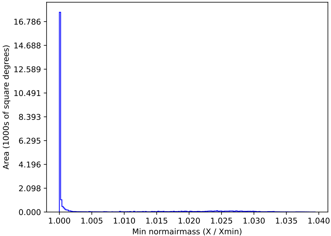
ddf_half_v3.4_10yrs All sky z band: Min normairmass
