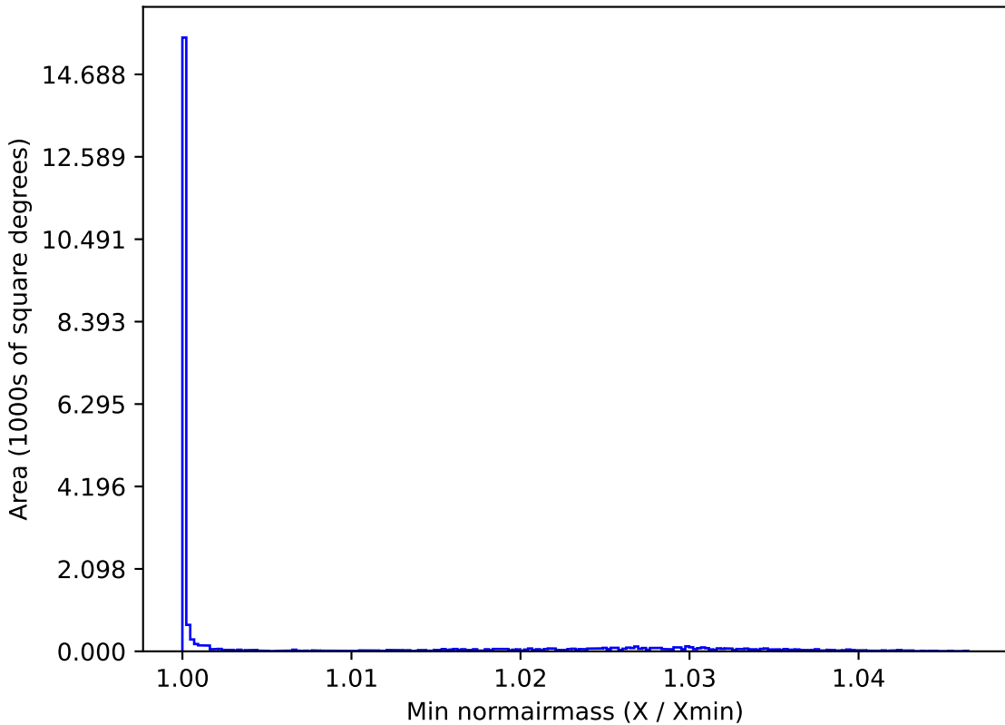
ddf_half_v3.4_10yrs All sky y band: Min normairmass
