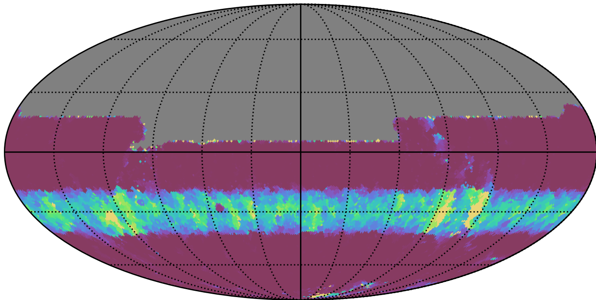
ddf_half_v3.4_10yrs All sky u band: Min normairmass
