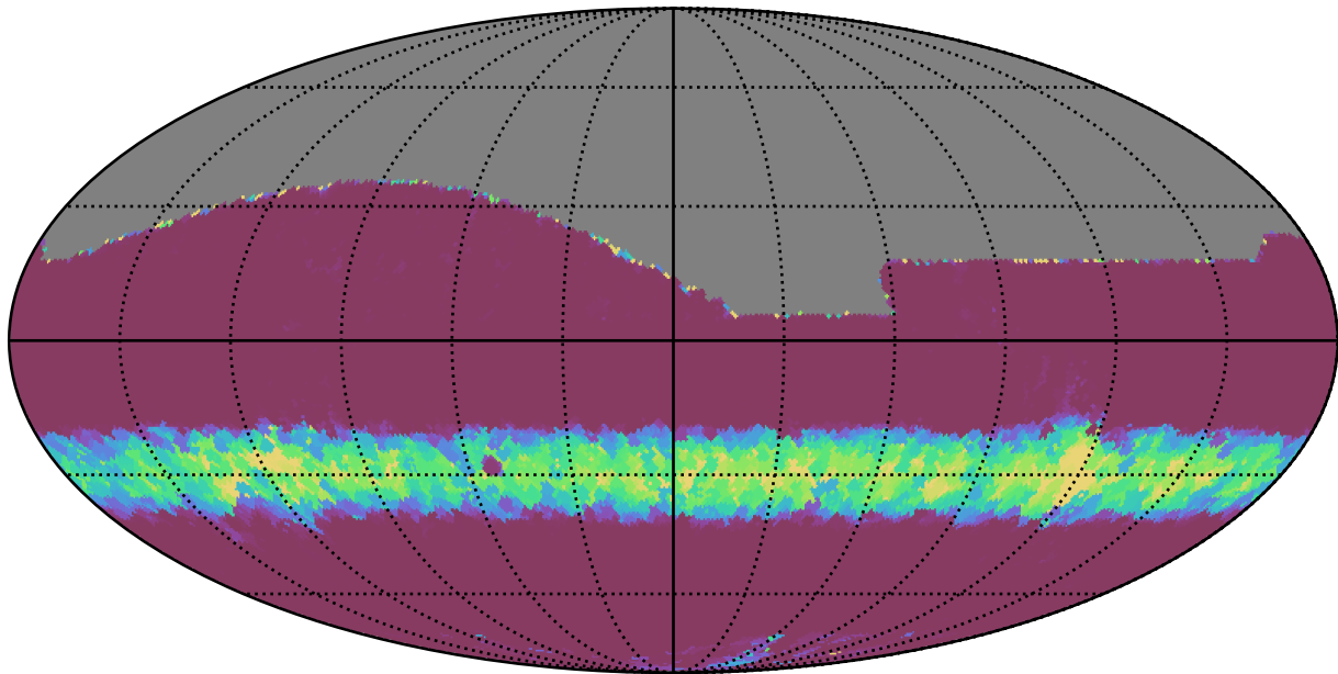
ddf_half_v3.4_10yrs All sky r band: Min normairmass
