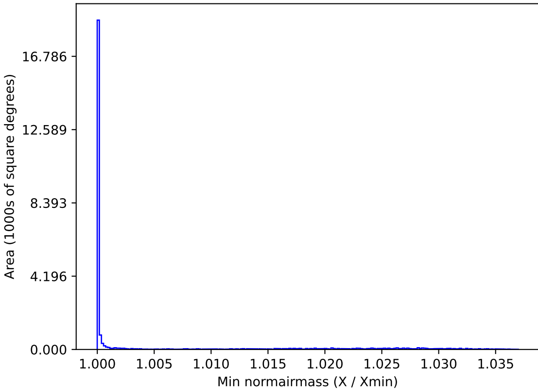
ddf_half_v3.4_10yrs All sky r band: Min normairmass
