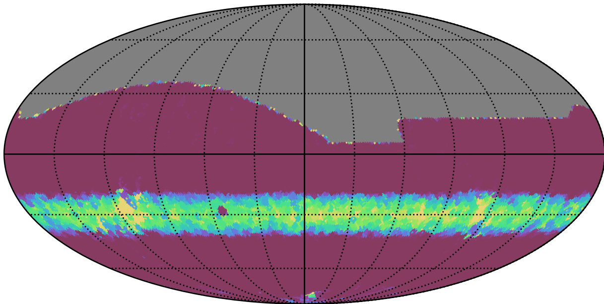
ddf_half_v3.4_10yrs All sky i band: Min normairmass
