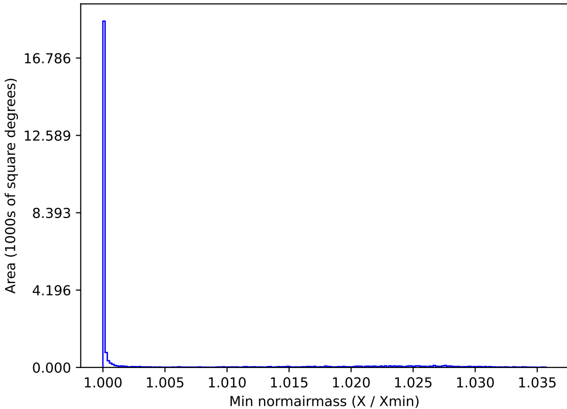
ddf_half_v3.4_10yrs All sky i band: Min normairmass
