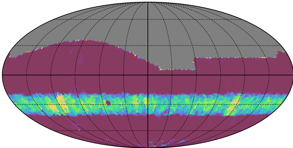
ddf_half_v3.4_10yrs All sky g band: Min normairmass
