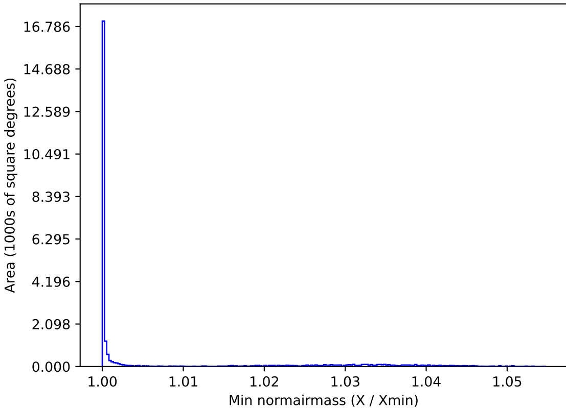
ddf_half_v3.4_10yrs All sky g band: Min normairmass
