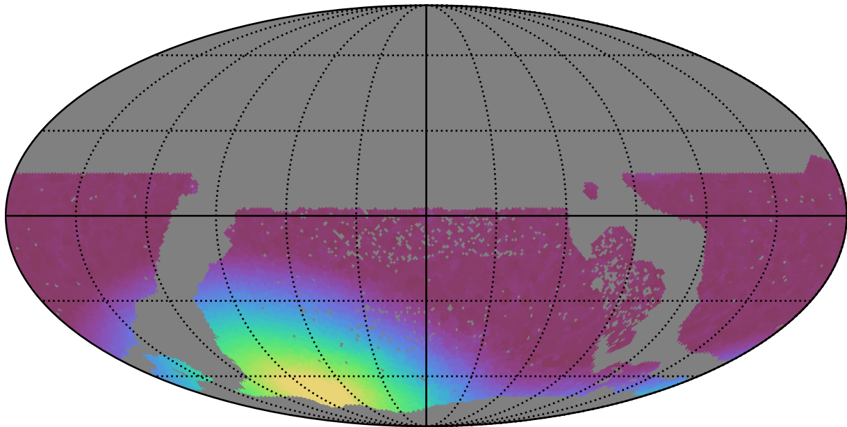
ddf_half_v3.4_10yrs WFD y band: Min moonDistance
