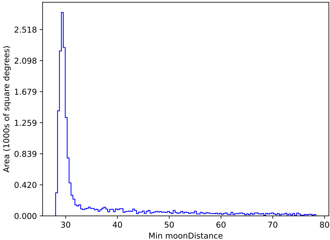
ddf_half_v3.4_10yrs WFD y band: Min moonDistance
