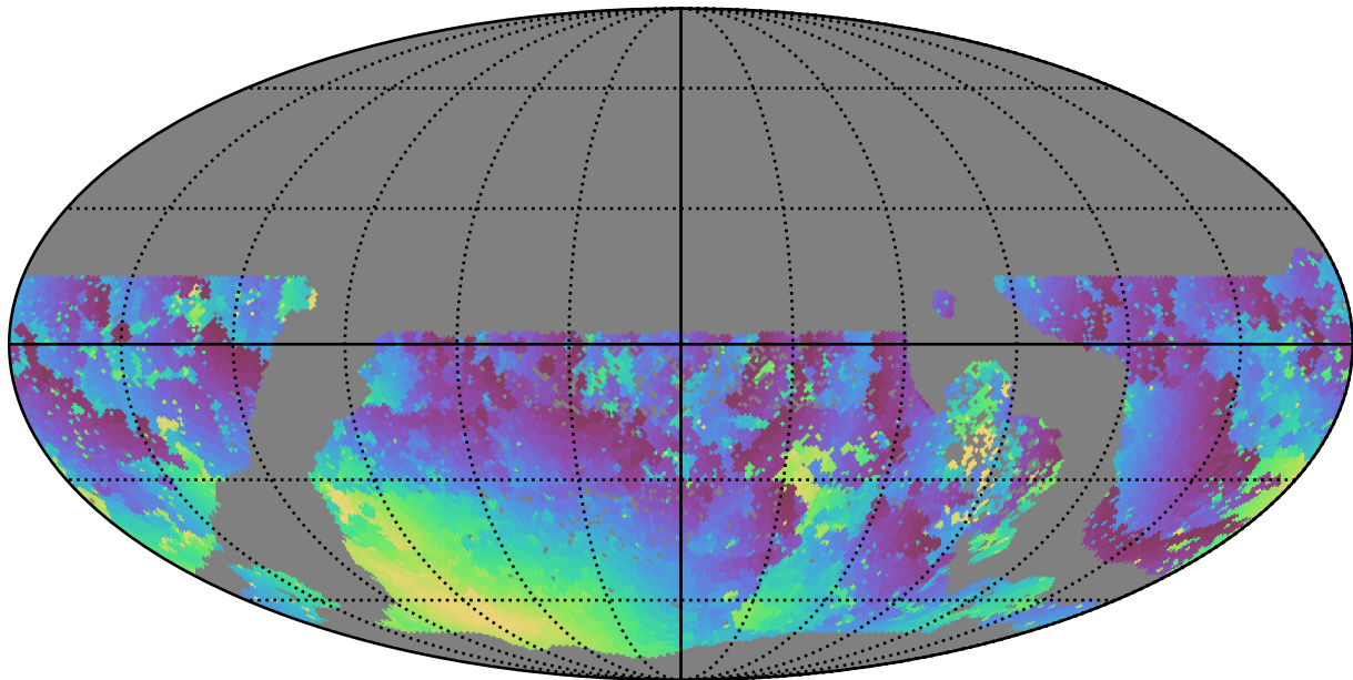
ddf_half_v3.4_10yrs WFD u band: Min moonDistance
