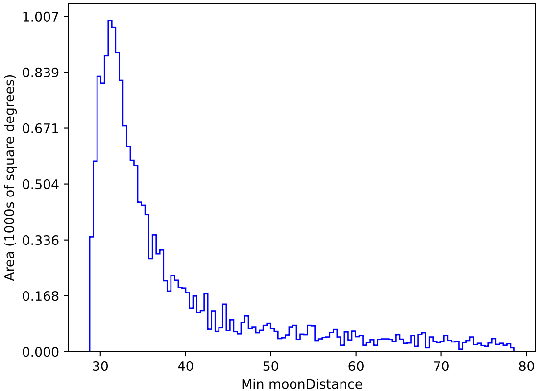
ddf_half_v3.4_10yrs WFD r band: Min moonDistance
