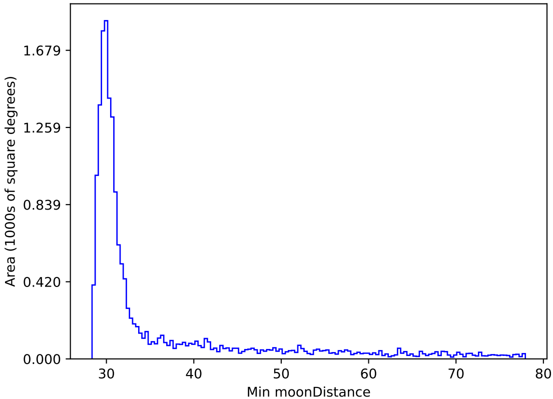
ddf_half_v3.4_10yrs WFD i band: Min moonDistance
