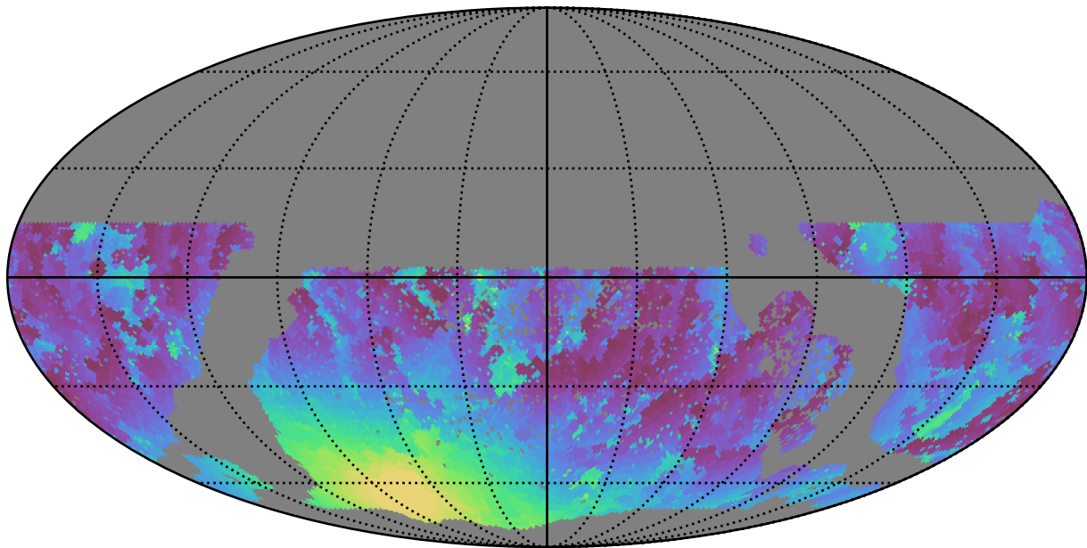
ddf_half_v3.4_10yrs WFD g band: Min moonDistance
