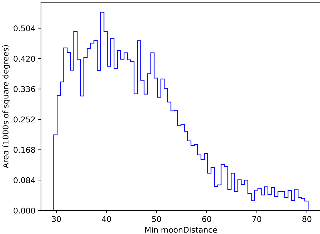
ddf_half_v3.4_10yrs WFD g band: Min moonDistance
