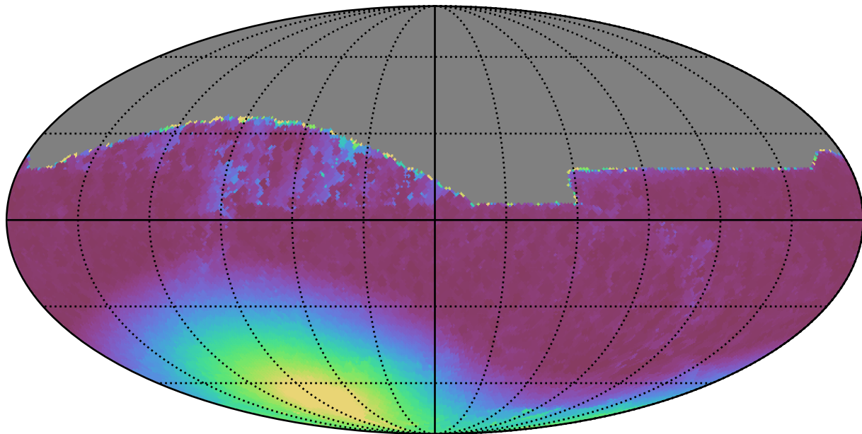
ddf_half_v3.4_10yrs All sky z band: Min moonDistance
