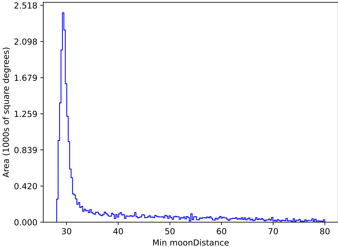
ddf_half_v3.4_10yrs All sky y band: Min moonDistance
