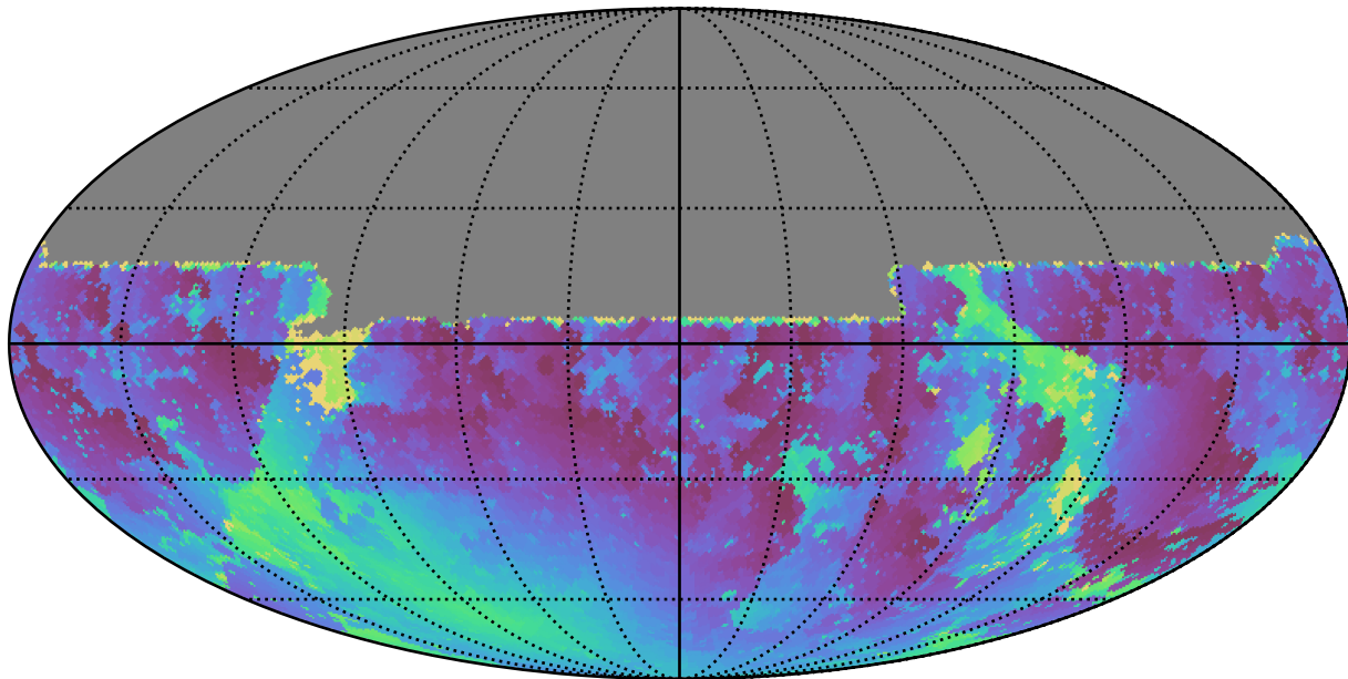
ddf_half_v3.4_10yrs All sky u band: Min moonDistance
