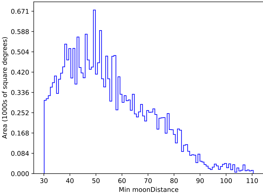
ddf_half_v3.4_10yrs All sky u band: Min moonDistance
