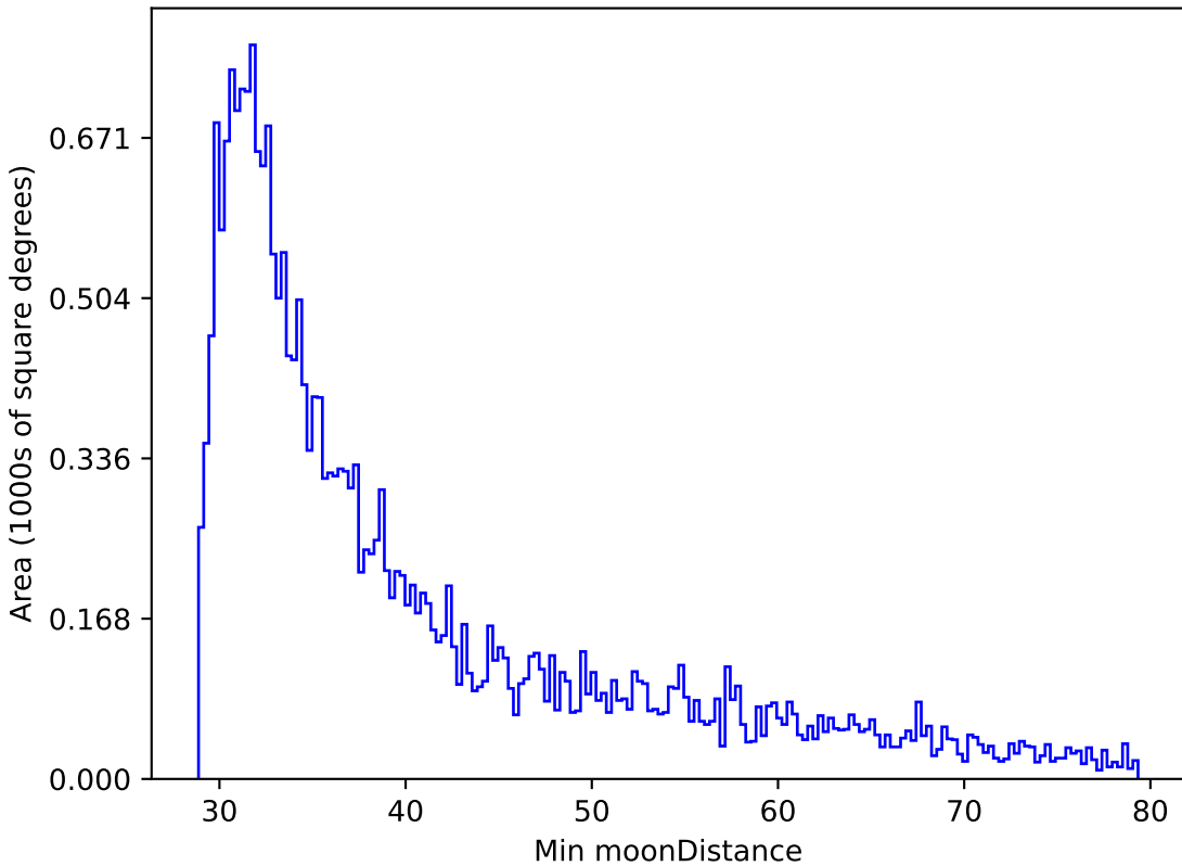
ddf_half_v3.4_10yrs All sky r band: Min moonDistance
