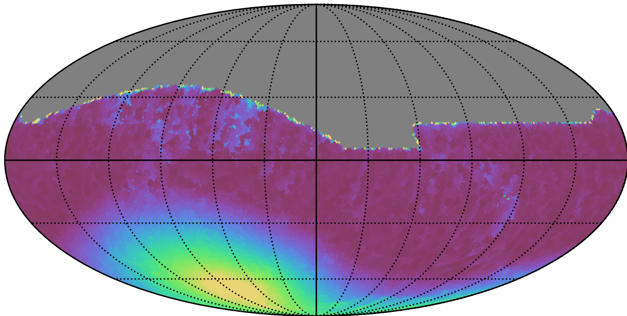
ddf_half_v3.4_10yrs All sky i band: Min moonDistance
