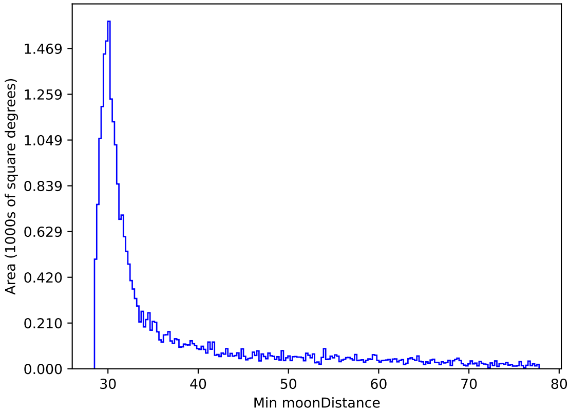
ddf_half_v3.4_10yrs All sky i band: Min moonDistance
