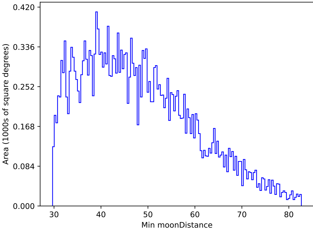
ddf_half_v3.4_10yrs All sky g band: Min moonDistance
