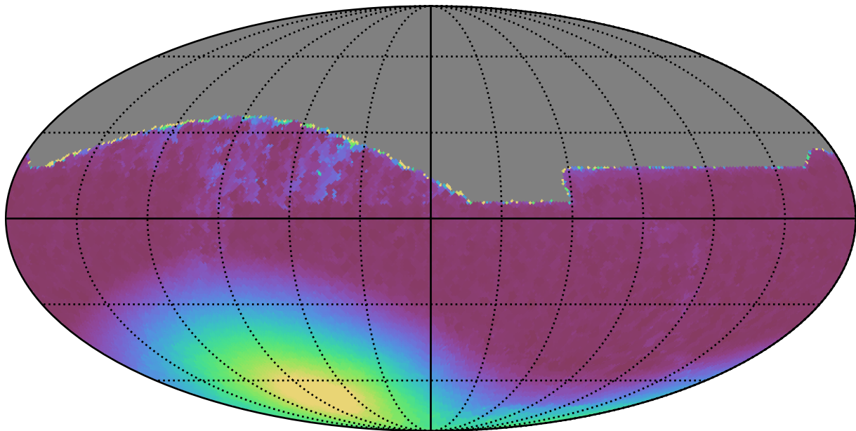
ddf_half_v3.4_10yrs All sky all bands: Min moonDistance
