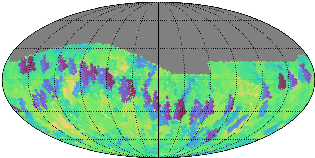
ddf_half_v3.4_10yrs Yr 1 z band: Min fiveSigmaDepth
